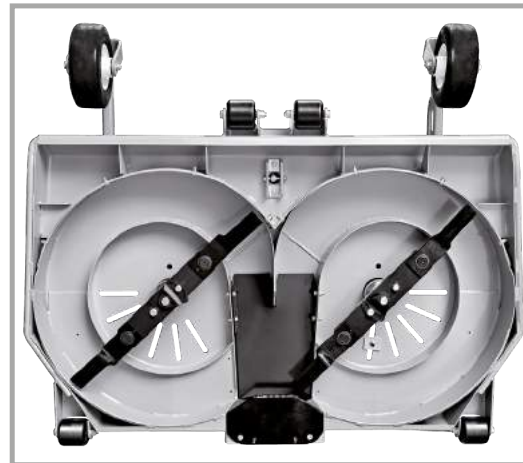
Mulching kit as a standard feature on cutting decks with collection
